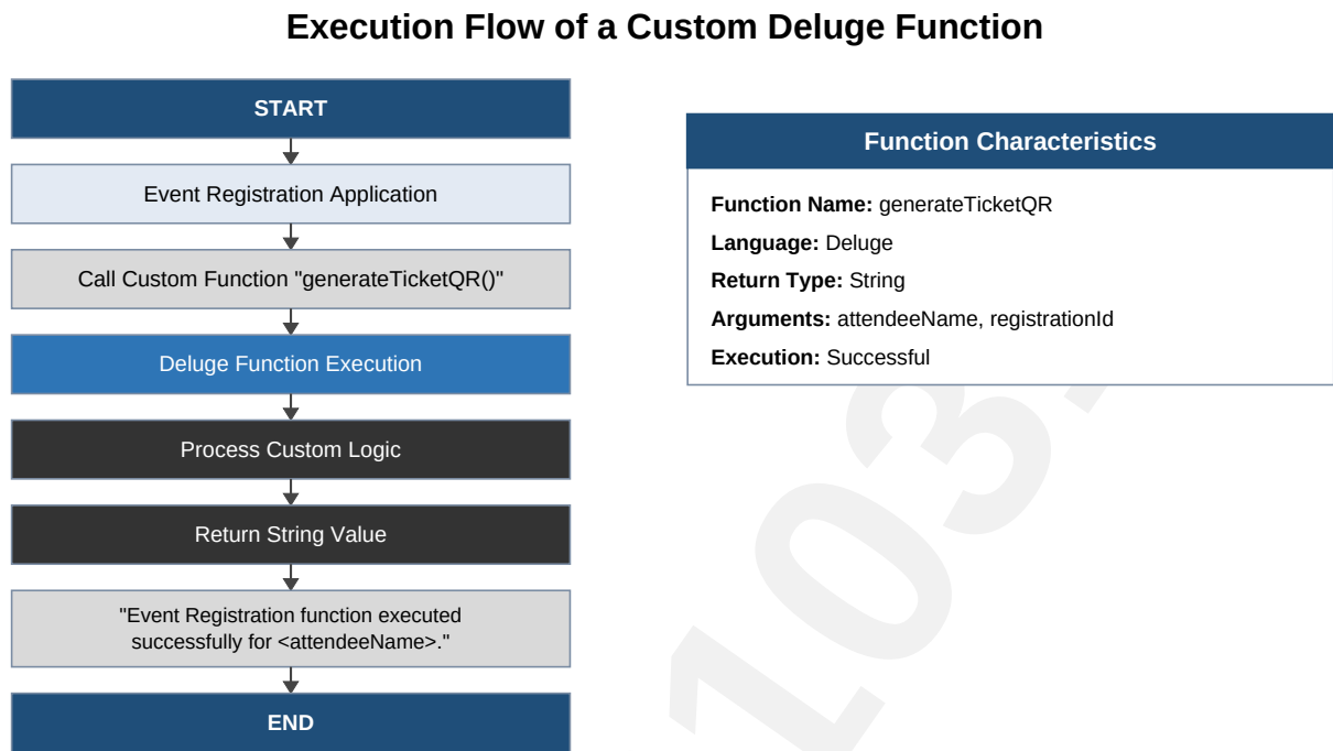
Figure 7: Execution Flow of a Custom Deluge Function (Supporting Diagram)
